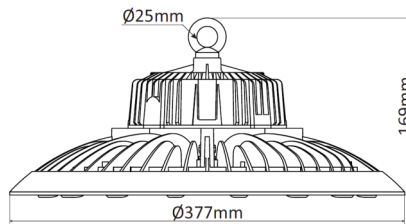
WSLI-UFOH150
