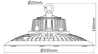
WSLI-UFOH100/KML -UFOH120
