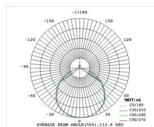
110° Glass cover
