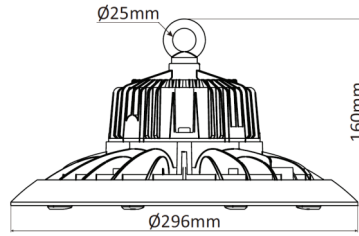
WSLI-UFOH080
