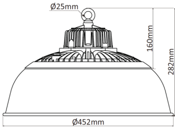
WSLI-UFOH100/KML -UFOH120
