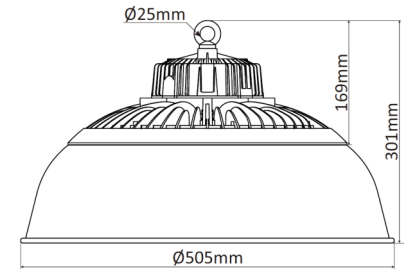
WSLI-UFOH150
