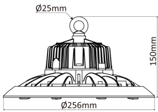
WSLI-UFOH050
