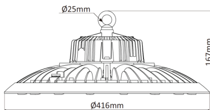
WSLI-UFOH200/KML -UFOH240
